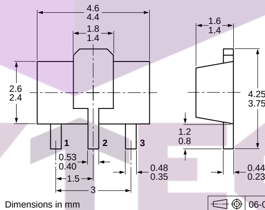
Fig 20. Package outline SOT89 (SC-62/TO-243)
